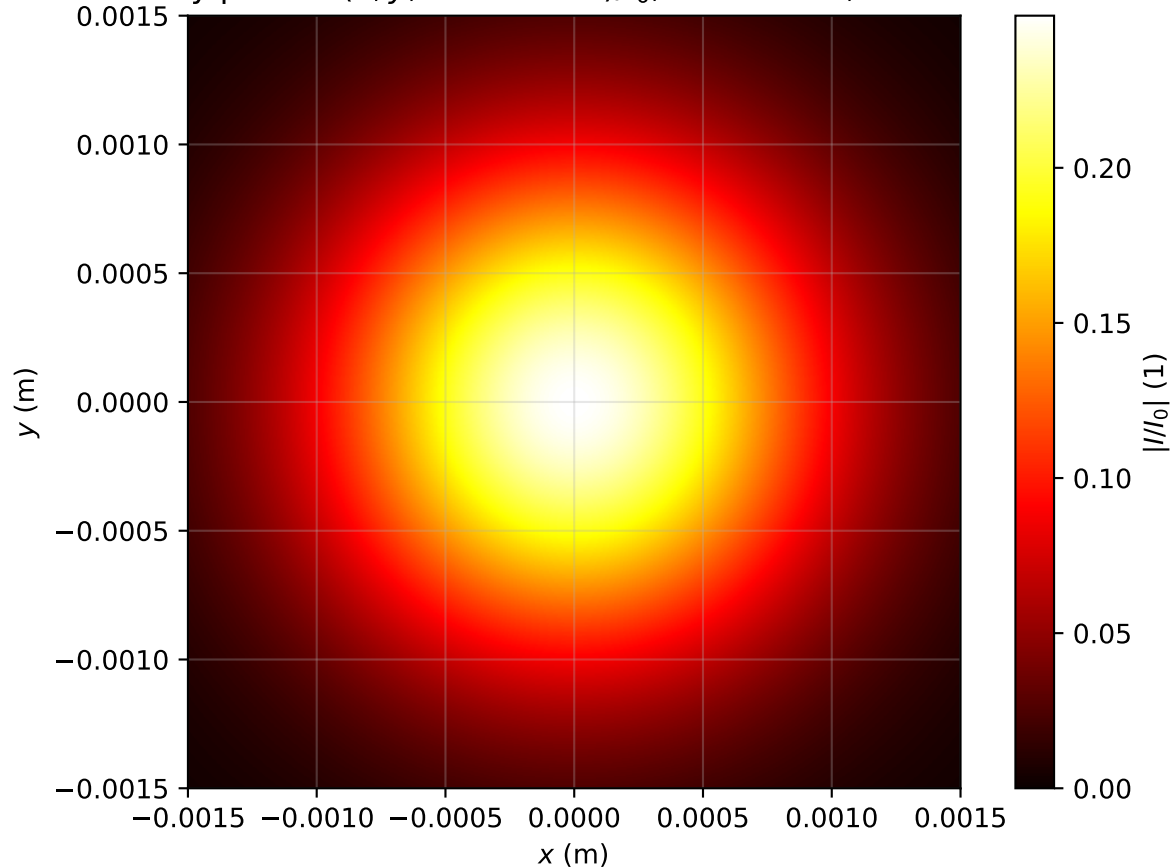
Intensity profile I(x, y, z = 3.981\text{m})/I_0 , P_{\text{in}}=0.2P_{\text{cr}} , artificial time
